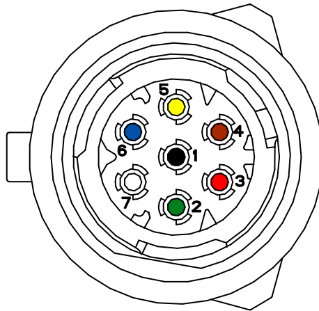
ORIENTATION OF DIN CONNECTOR AS VIEWED EXTERNALLY ON LAMP
