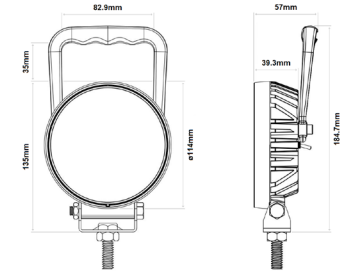
711.034 Handle & Switch
