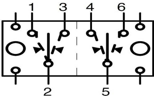
CIRCUIT DIAGRAM
